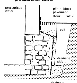
⑪ Repairs to soil side of masonry foundations
